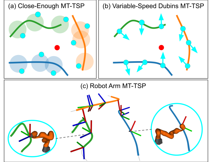
Fig. 4. IRG-PGLNS sampling strategy applied to three MT-TSP variants. (a) Close-Enough MT-TSP: samples lie on disc boundaries. (b) Variable-Speed Dubins MT-TSP: a sample point's position matches the target's position at the sampled time, but the sample point's heading is random. (c) Robot Arm MT-TSP: each sample point is an arm configuration-time pair, where the end-effector pose for the arm configuration must match the target's pose at the sampled time. Target poses at sampled times are shown with reference frames.
