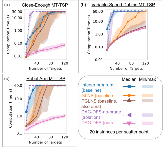
Fig. 12. Comparison of computation time for methods for solving the GTSP on the first set of sample points. Our DAG-DFS method, used in all the IRG variants, scales better with the number of targets than the other methods.
