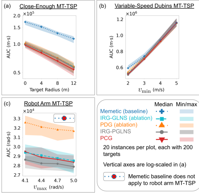
Fig. 10. (a) Varying target radius in Close-Enough MT-TSP. PCG has smaller min, median, and max AUC than all other planners for all radii. (b) Varying v_{\min} in Variable-Speed Dubins MT-TSP. IRG-PGLNS and PCG perform similarly to each other and have smaller min, median, and max AUC than baselines and ablations for v_{\min} \leq 4 . (c) Varying v_{\max} in Robot Arm MT-TSP. IRG-PGLNS has smaller median and max AUC than all other planners for all v_{\max} .
