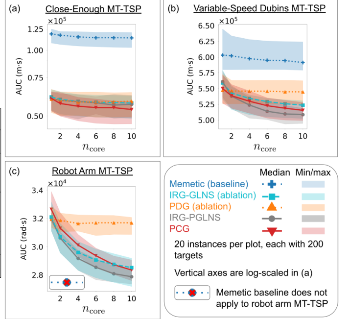
Fig. 9. Varying the number of cores used by each algorithm. Methods' AUC values differ when they all use 1 core because they use different values of n_{rand} and \alpha_{term} . Each planner's AUC tends to decrease as we increase the number of cores, with PDG and the memetic algorithm showing smaller decreases.
