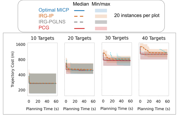
Fig. 11. Testing IRG variations against optimal MICP solver [22] on “linear” MT-TSP instances, as defined at the beginning of Section VIII. For instances with 10 and 20 targets, the optimal MICP found the optimal solution within the 1 min time limit, but on the instances with 30 and 40 targets, it did not certify that it found the optimum in any instance. IRG-PGLNS and PCG converge closely to the optimum for 10 and 20 targets and scale better with the number of targets than the optimal MICP and IRG-IP.
