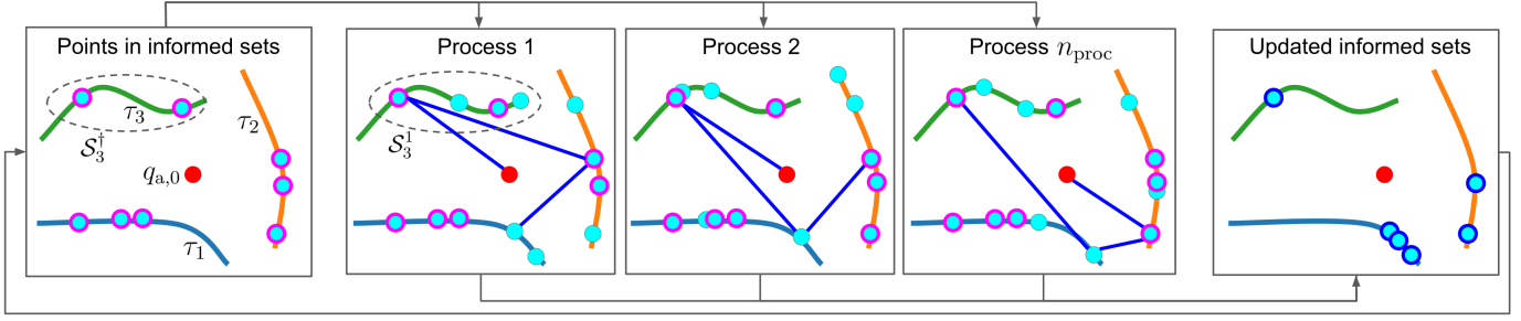
Fig. 5. Illustration of an iteration of trajectory improvement in PCG. The main process maintains an informed set of points \mathcal{S}_i^\dagger for each target i . Points in the current iteration's informed sets are outlined in pink. Each child process j generates a set of sample points \mathcal{S}_i^j for each target i , containing the points from the current \mathcal{S}_i^\dagger and random points unique to process j . Each child process then solves a GTSP, finding a sequence of points beginning at q_{a,0} visiting one point per target. The main process then updates the informed set for each target i to contain all visited points associated with target i from all child processes.
