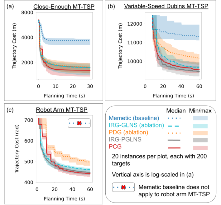
Fig. 7. Cost vs. time for three MT-TSP variants, in instances with 200 targets. IRG-PGLNS and PCG find notably lower-cost solutions than the baseline and ablations, except for the Close-Enough MT-TSP (a), where IRG-PGLNS outperforms the memetic baseline while performing similarly to the ablations.
